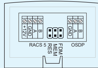
MCI-3 OSDP comm interface
