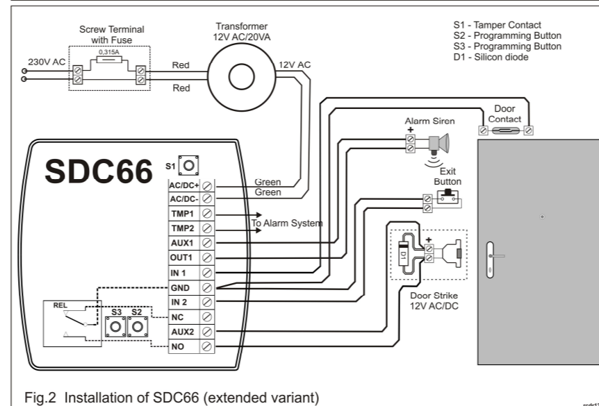
Fig.2 Installation of SDC66 (extended variant)
