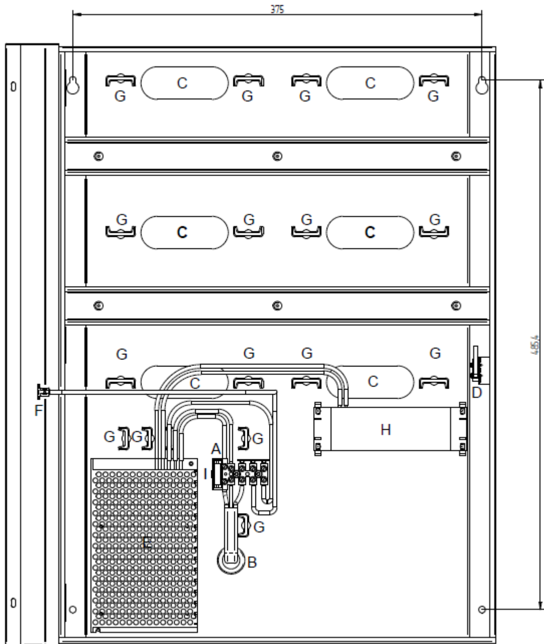
Fig. 2 Internal view of ME-43 enclosure: A: Mains Supply Terminal Blocks with Fuse; B: Main Supply Entry Hole with Protective Sleeve; C: Low Voltage Connection Holes; D: Tamper Contact; E: Power Supply Module; F: Door PE Connector; G: Cable Tie Eyelets; H: Power Distribution Module
