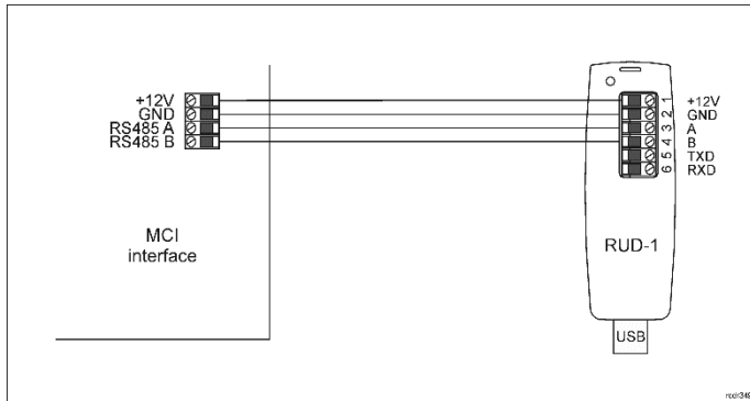
Fig. 1 Connection of the MCI-3 to RUD-1 interface for configuration
