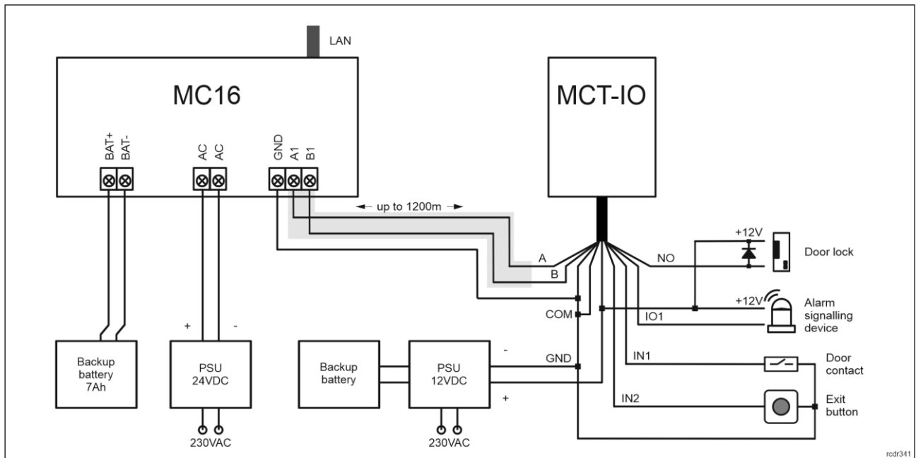
Fig. 7 Typical connection diagram for the -IO version terminal and MC16 access controller
