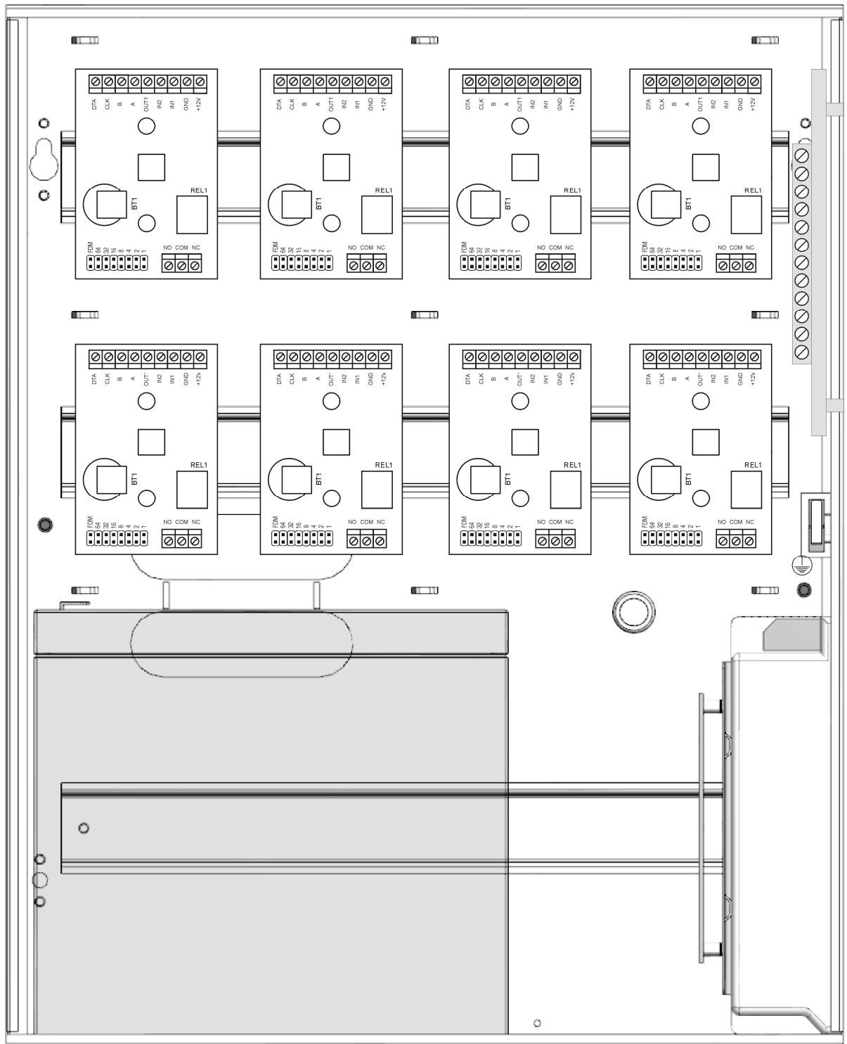
Fig. 3 PR102DR-BRD controllers installed inside ME-2-D (example)
