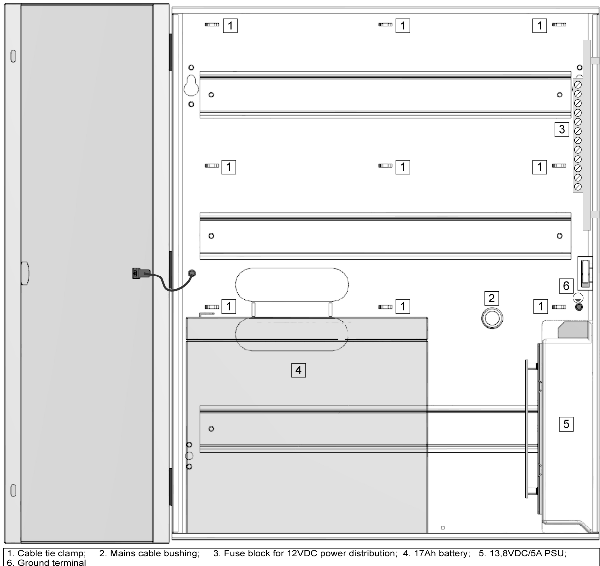
Fig. 1 Inside view of ME-2-D set with buffer PSU, fuse block and optional 12V/17Ah battery
