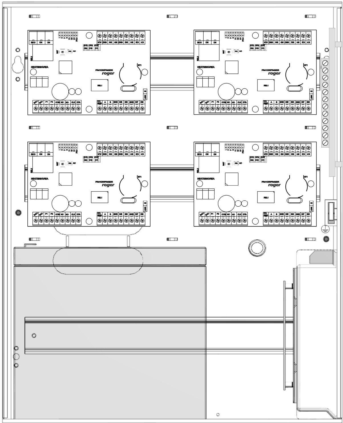
Fig. 2 PR402DR-12VDC-BRD controllers installed inside ME-2-D (example)
