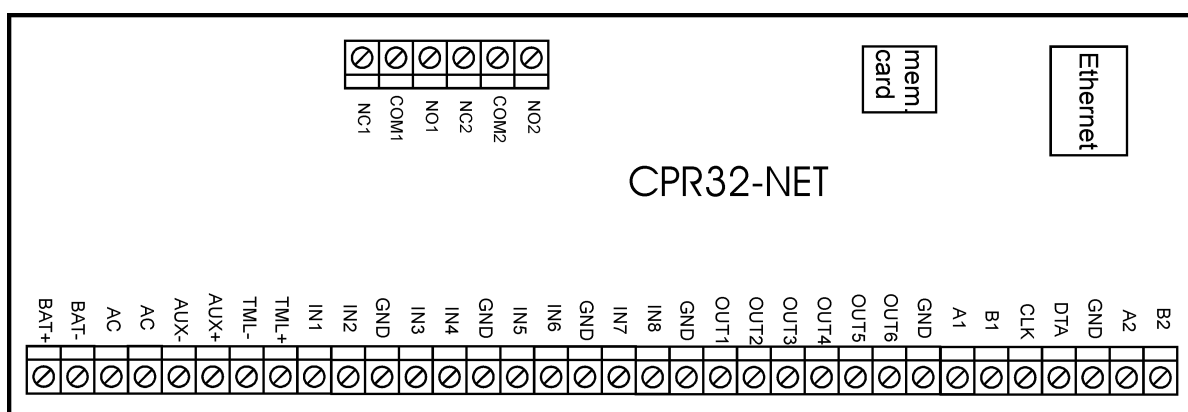
Fig. 1 CPR32-NET network controller board
