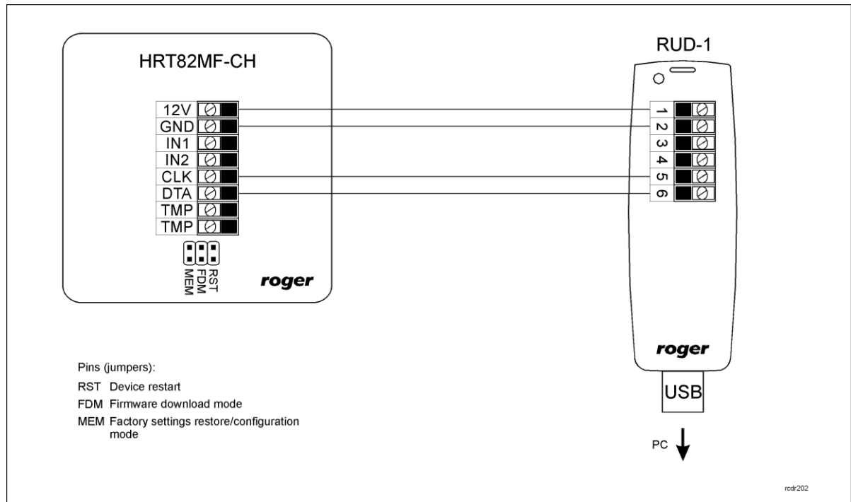
Fig. 6 HRT82MF-CH and RUD-1 connection
