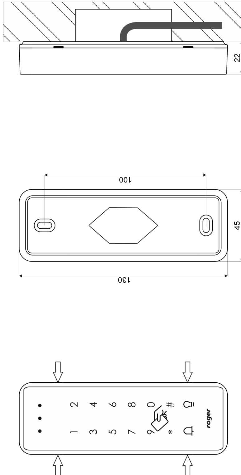
MCT84M terminal
