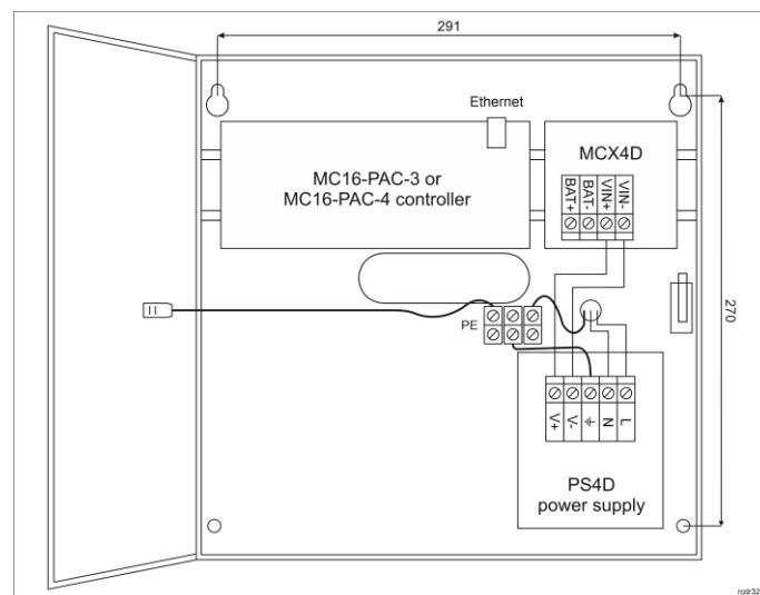
Fig. 1 MC16-PAC-3-KIT or MC16-PAC-4-KIT
