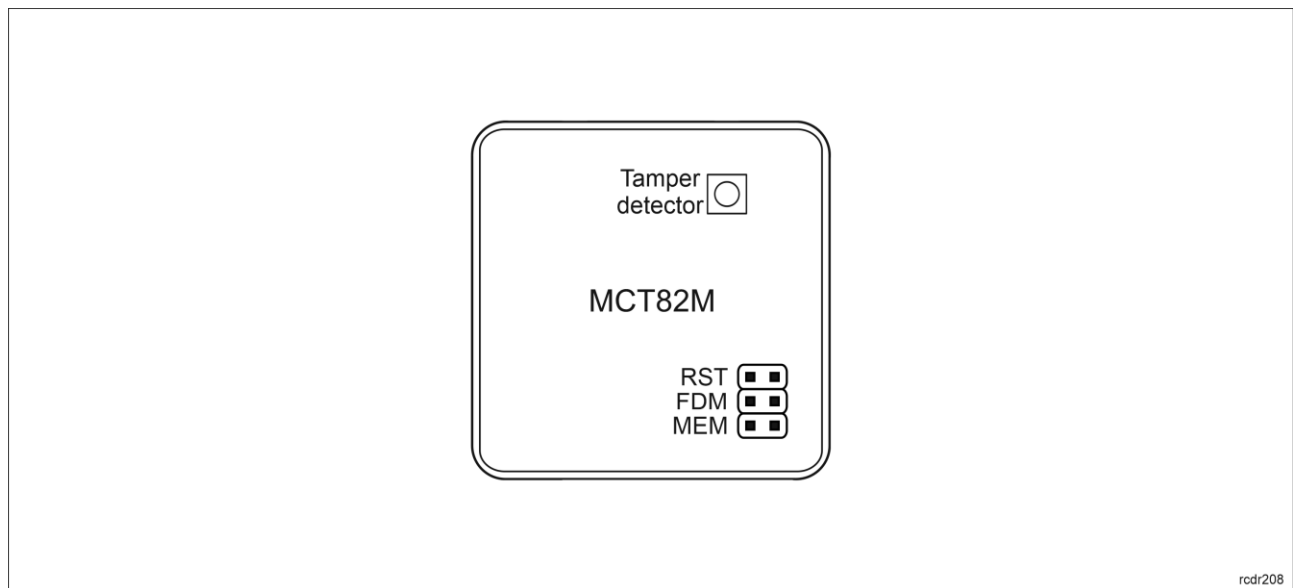
Fig. 6 Programming jumpers
