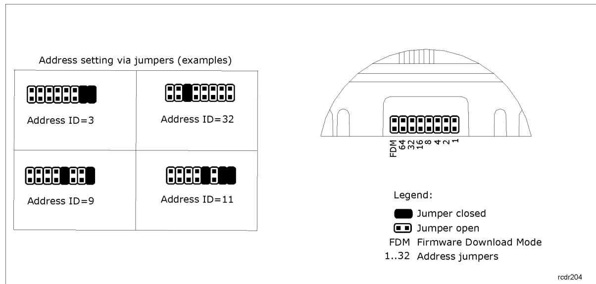
Fig. 9 Addressing jumpers
