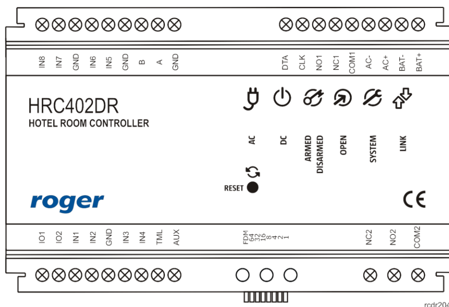
Fig. 1 HRC402DR controller
